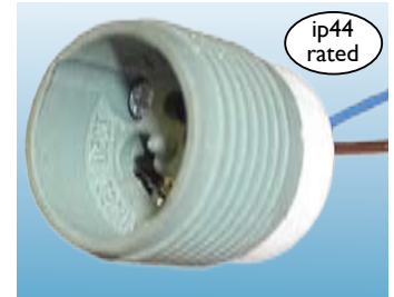
2325 ip44 lamp holder with threaded entry - threaded
